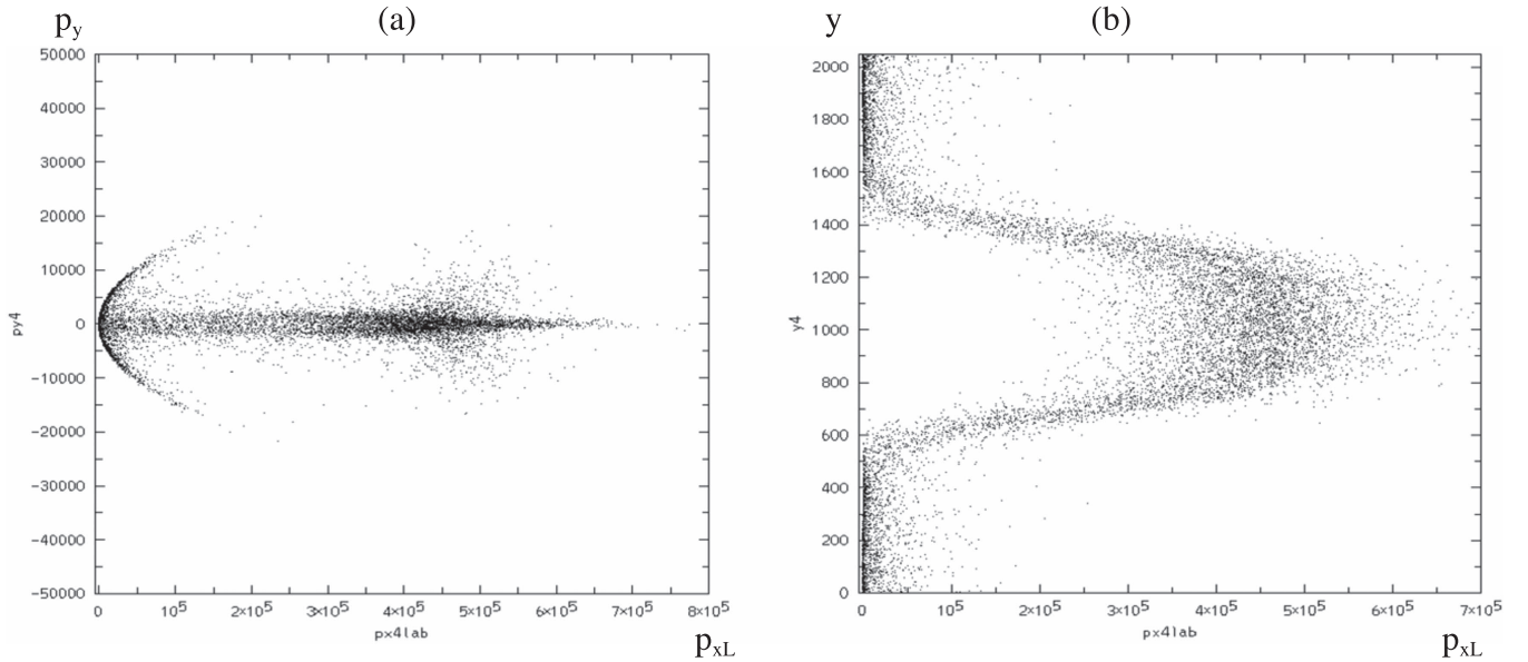
Figure 8. Phase plots of spine electrons for the pure e–ion run of Figure 2(a) at t\omega_c = 10,000 , after Lorentz boosting \mathbf{p}_x to the “laboratory frame” in which the sheath is initially at rest: (a) p_{xL} vs. p_y and (b) p_{xL} vs. y\omega_c/c . By this time, many of the spine electrons have diffused into the sheath located at y\omega_c/c < 500 and y\omega_c/c > 1500 of panel (b), and are decelerated and thermalized. These “cross over” electrons form the bow-shaped, low-energy population shown in panel (a), while the arrow-shaped high-energy population corresponds to electrons remaining in the spine ( 500 < y\omega_c/c < 1500 of panel (b)). Note the narrow beaming of the highest-energy electrons in panel (a), which are accelerated up to \sim 0.5 TeV. The broadening of the p_y distribution around p_x \sim 5 \times 10^5 in panel (a) is caused by mid-plane collisions, which is likely an artifact of the small PIC box.
