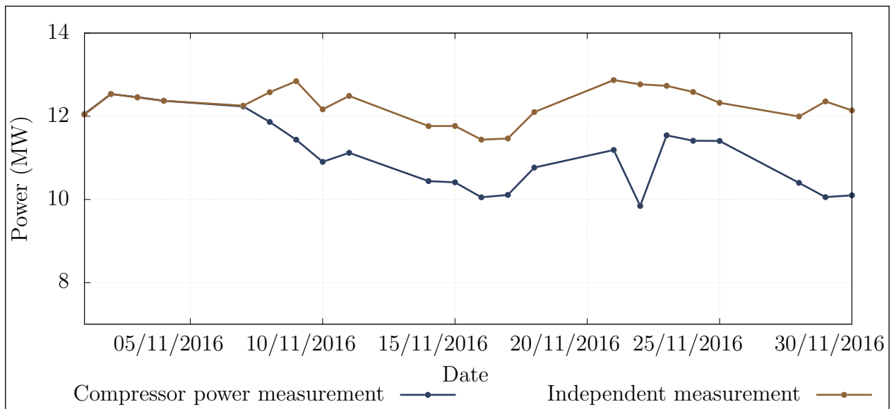
Figure 4.22: Comparison using alternative power sources
