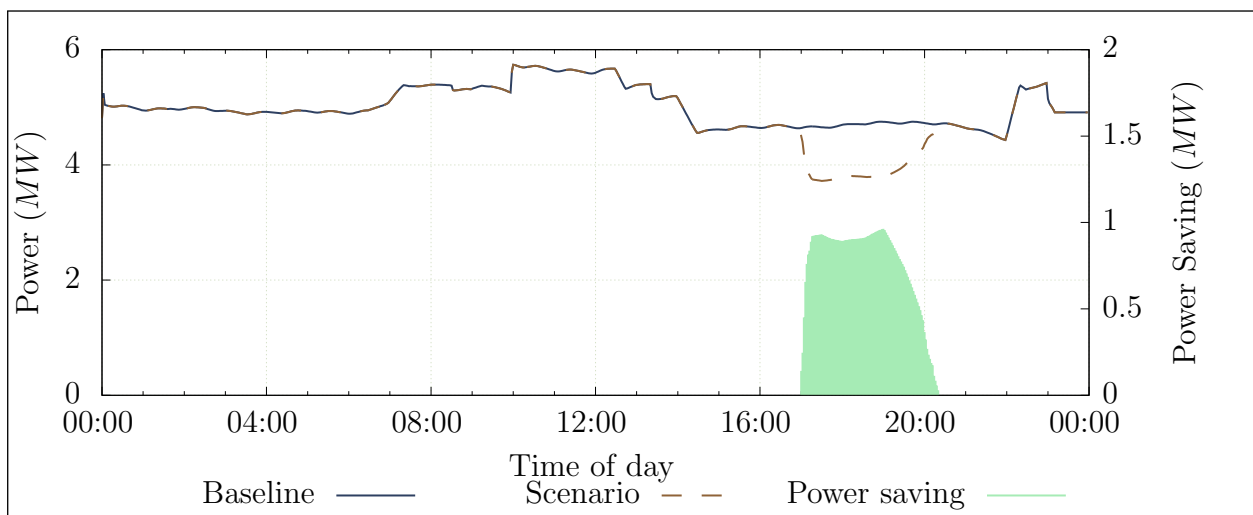
Figure 4.7: Scenario 2 - Simulated peak-time power reduction
