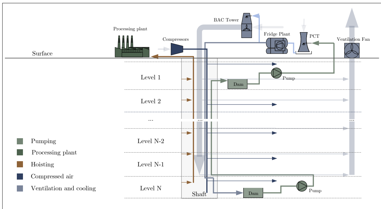
Figure 1.2: Schematic representation of the mining processes
