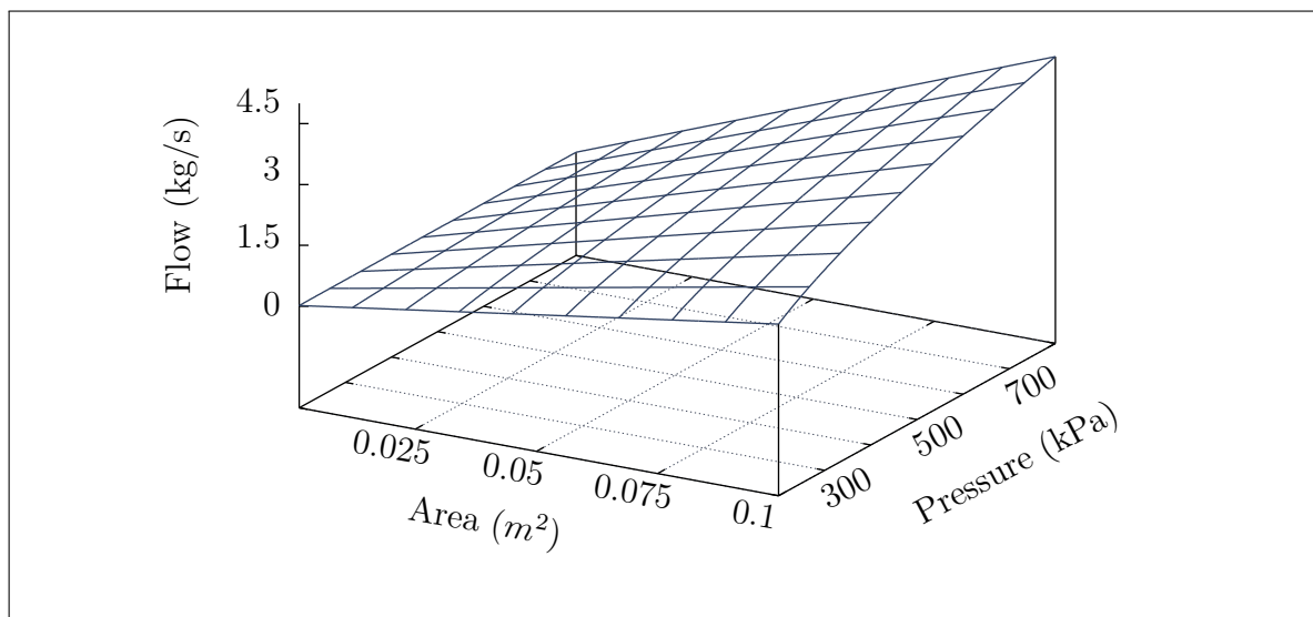
Figure 2.4: The flow due to leakage as a function of inlet pressure and leakage area 1
