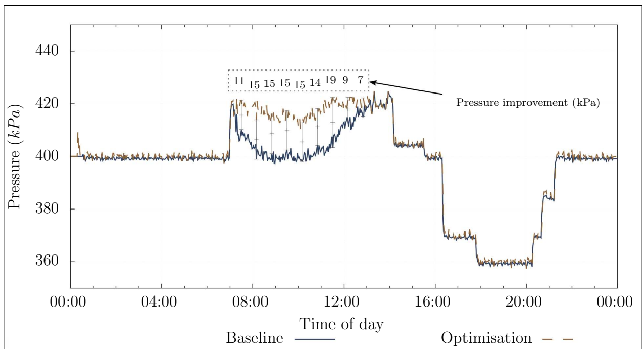
Figure 4.15: Baseline system pressure relative to system pressure when refuge bay leaks were reduced
