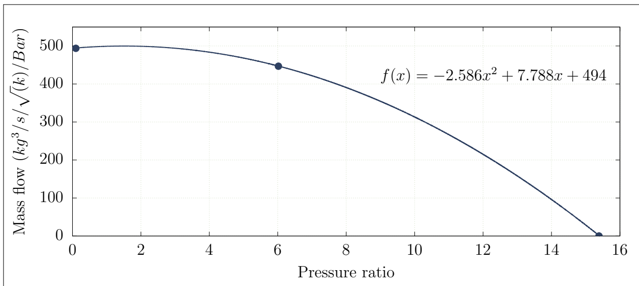
Figure 3.7: Estimating the characteristic curve of a compressor by fitting a quadratic function to points of operation
