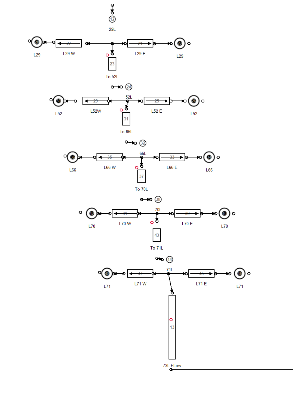
Figure I.5: Mine B simulation schematic – Main shaft air users
