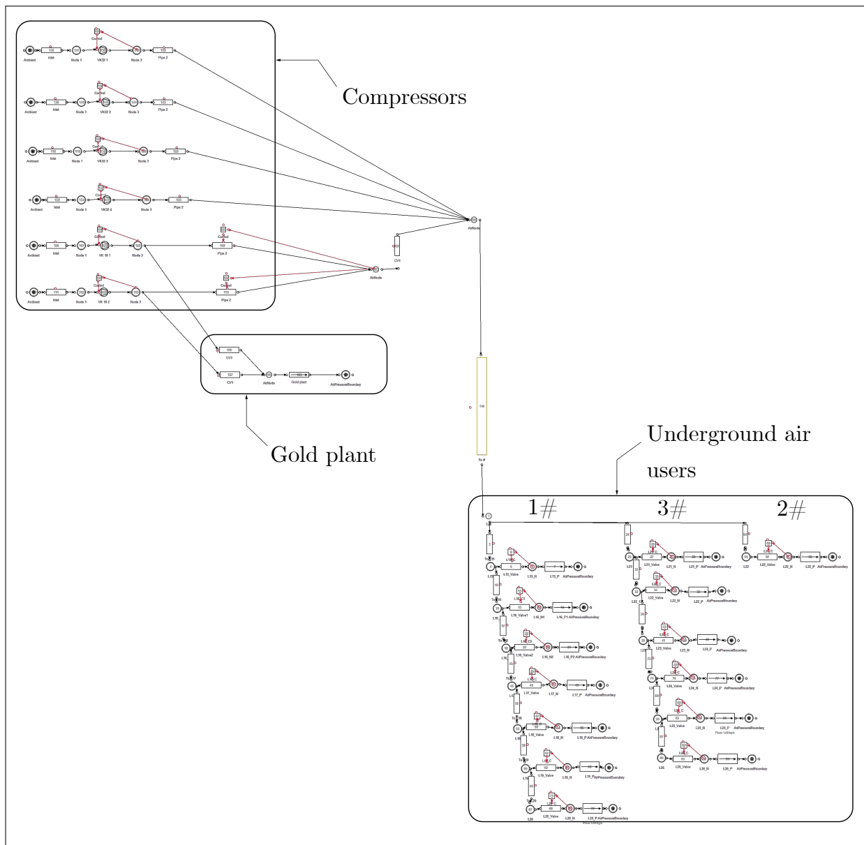
Figure I.1: Schematic representation of Mine A's compressed air simulation
