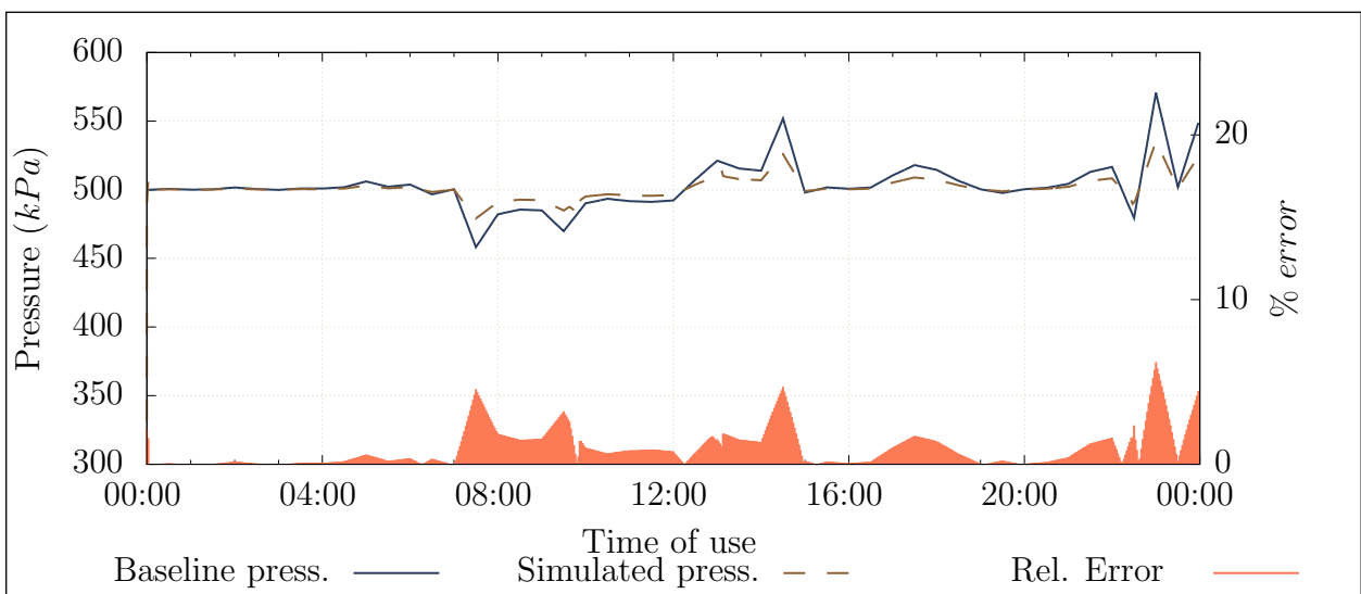
Figure 4.5: Simulated pressure compared to the actual measurement
