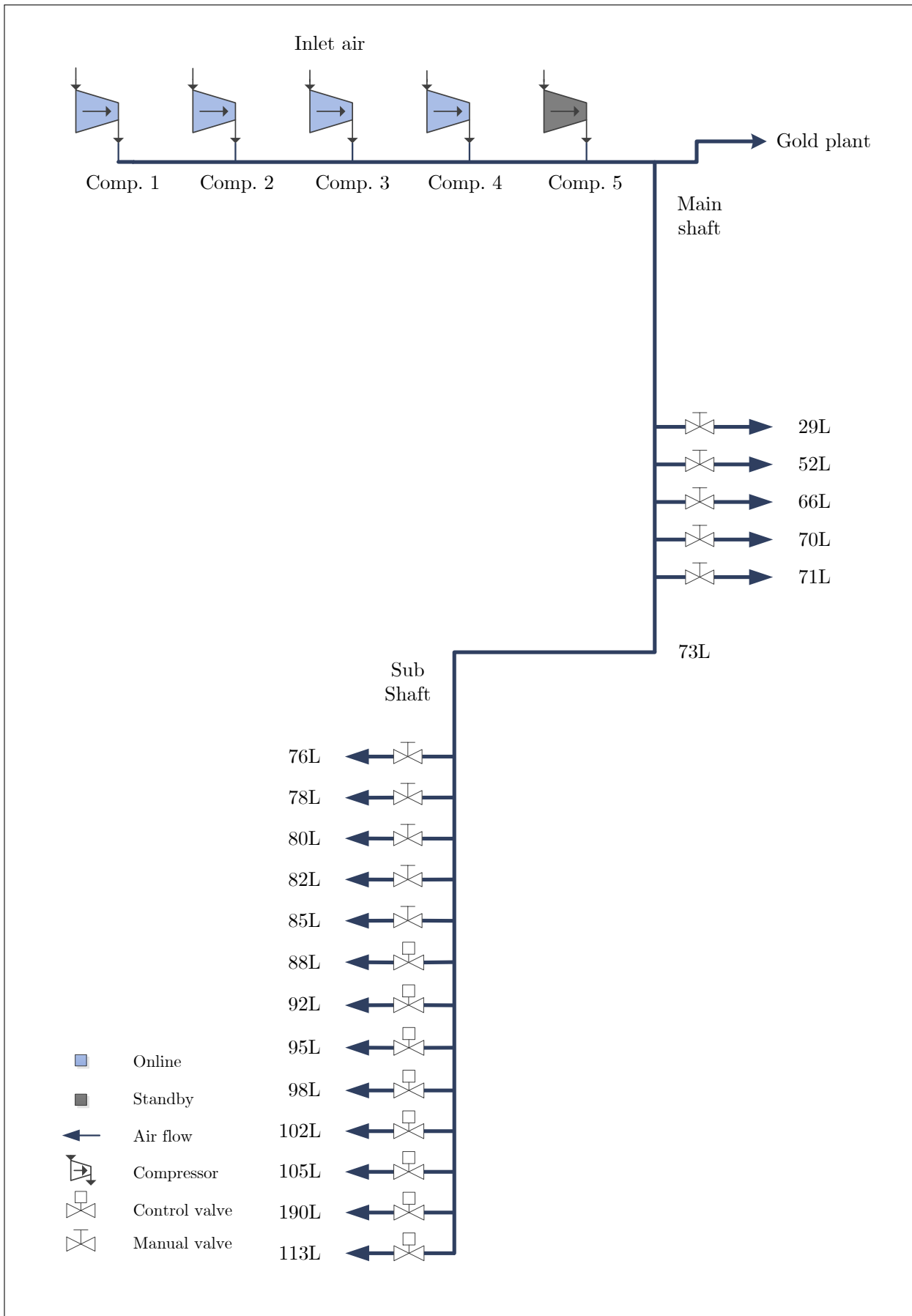
Figure 4.9: Process schematic of the compressed air network
