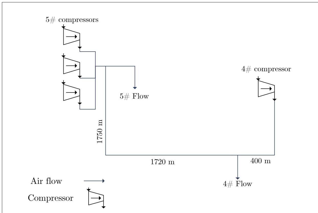
Figure 2.11: Compressor relocation simulation model (adapted from Bredenkamp [29])
