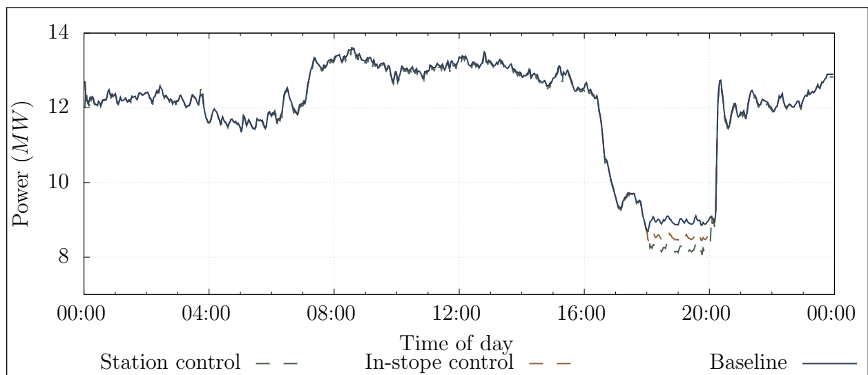
Figure 4.18: Comparing simulated flow interventions on 105 Level
