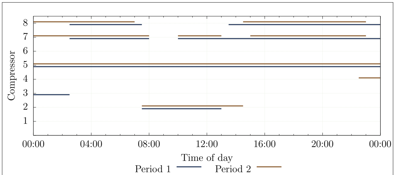
Figure 3.15: Example of two baseline periods, showing a changed compressor schedule
