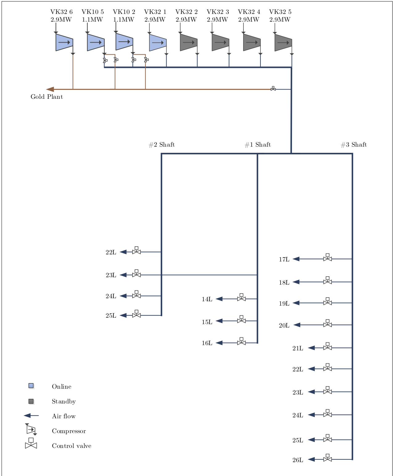
Figure 4.1: Simplified process flow chart of the compressed air network
