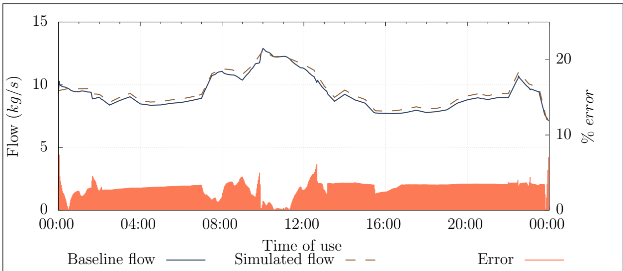
Figure 4.4: Simulated flow compared to the actual measurement
