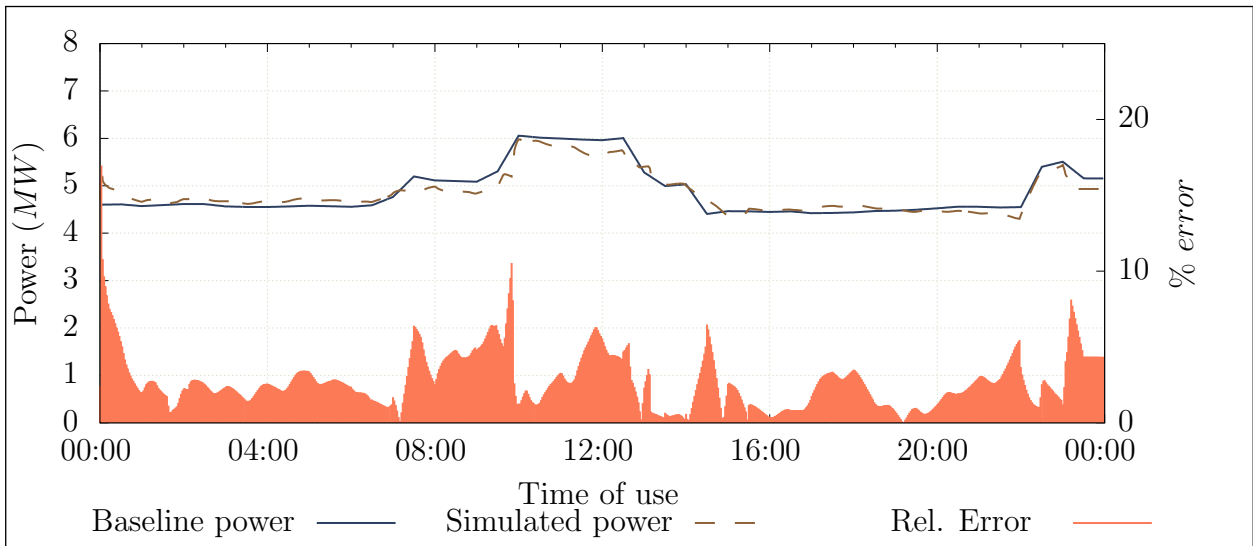
Figure 4.3: Simulated power compared to the actual measurement
