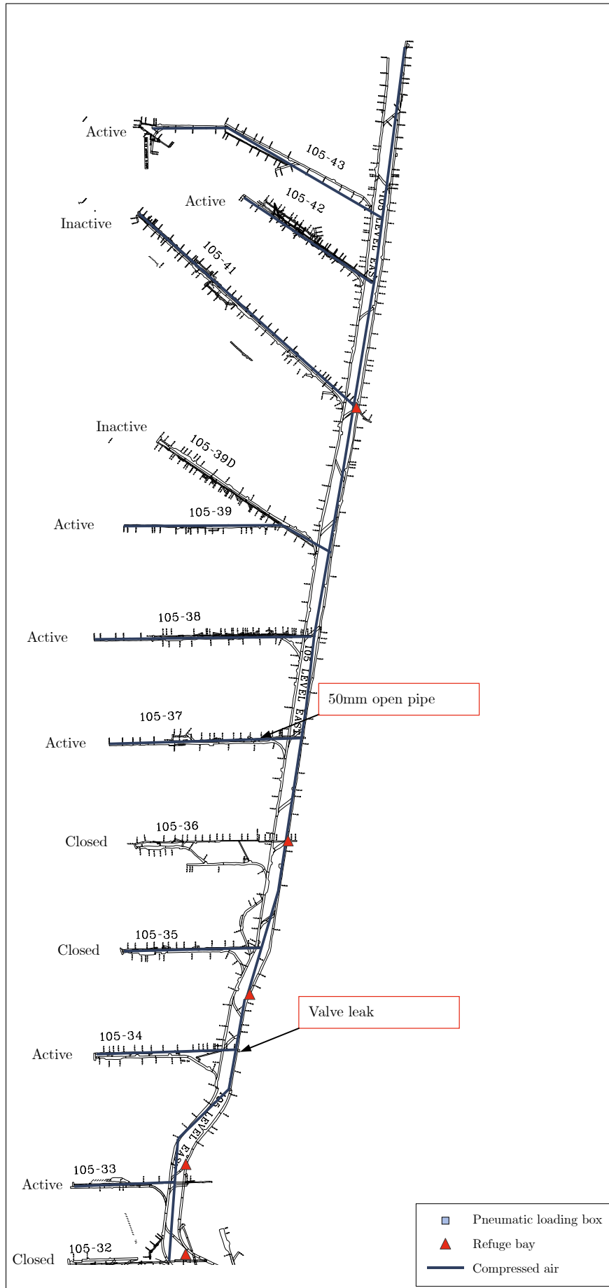
Figure IV.2: 105 Level investigation – West operations
