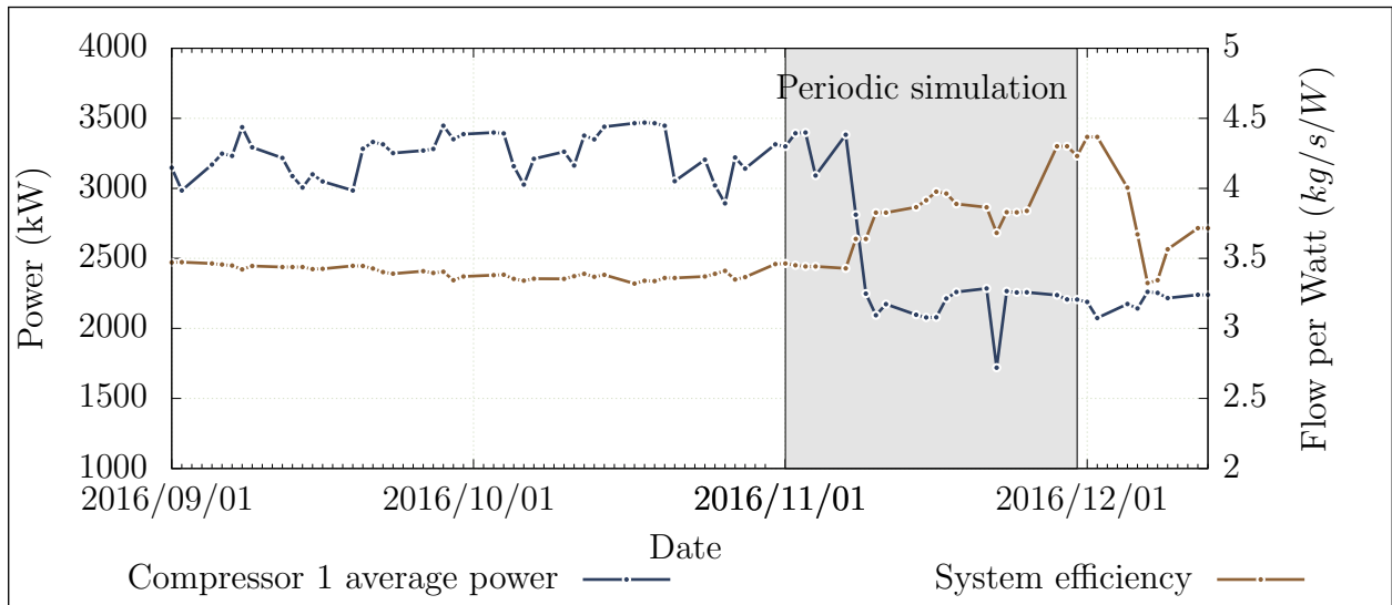
Figure 4.21: Supply efficiency and Compressor 1's average power output over the time of the periodic analysis
