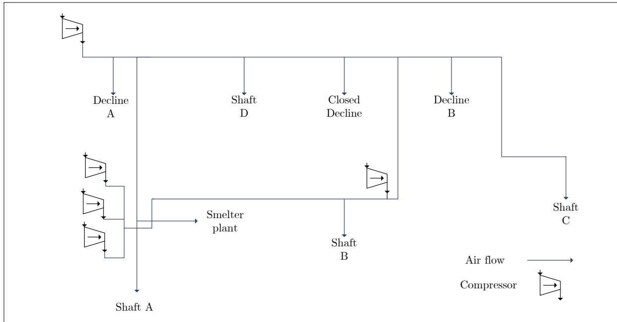
Figure 2.12: Simplified compressed air ring model (adapted from Pascoe [32])
