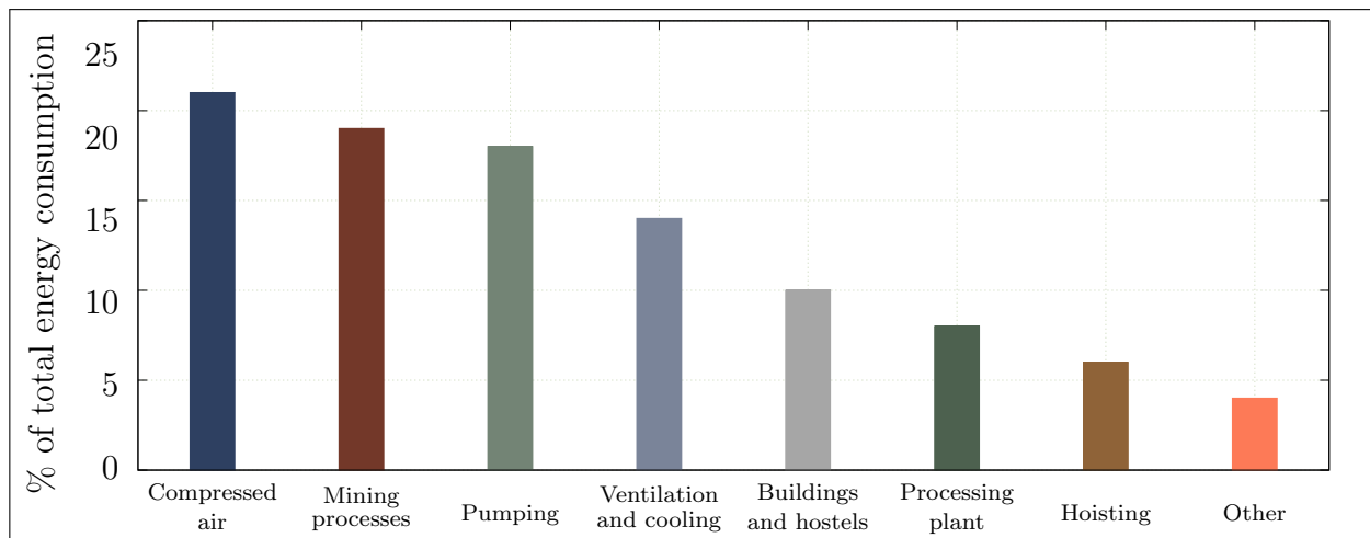
Figure 1.3: The percentage of energy consumption for each type of mining system [5]
