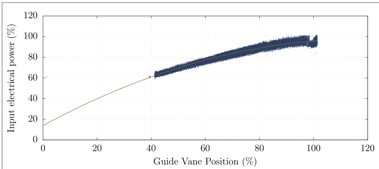
Figure 3.13: Modelling the compressor control from a guide vane 1
