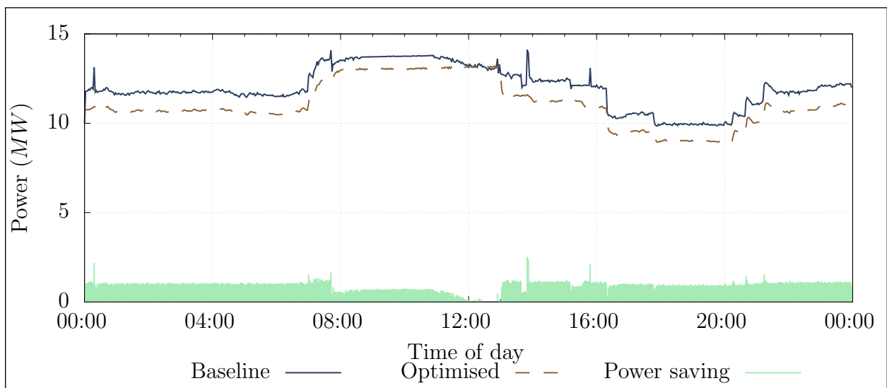
Figure 4.14: Baseline system power compared to system power when refuge bay leaks were reduced
