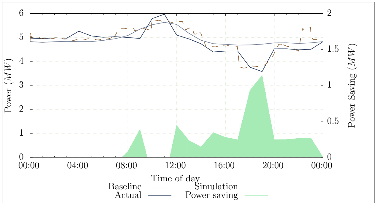
Figure 4.8: Actual power savings achieved on the system
