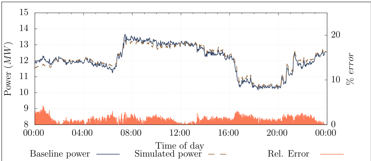
Figure 4.10: Simulated power compared to the actual measurement
