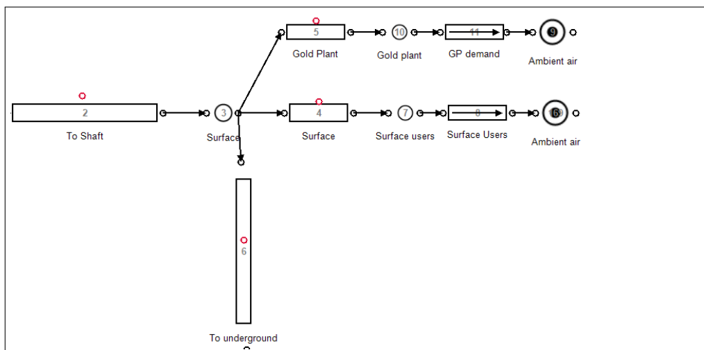
Figure I.4: Mine B simulation schematic – Surface air users
