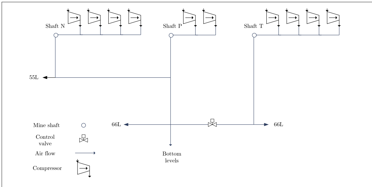
Figure 2.13: Simulation model for a complex air network (adapted from Maré et al. [19])
