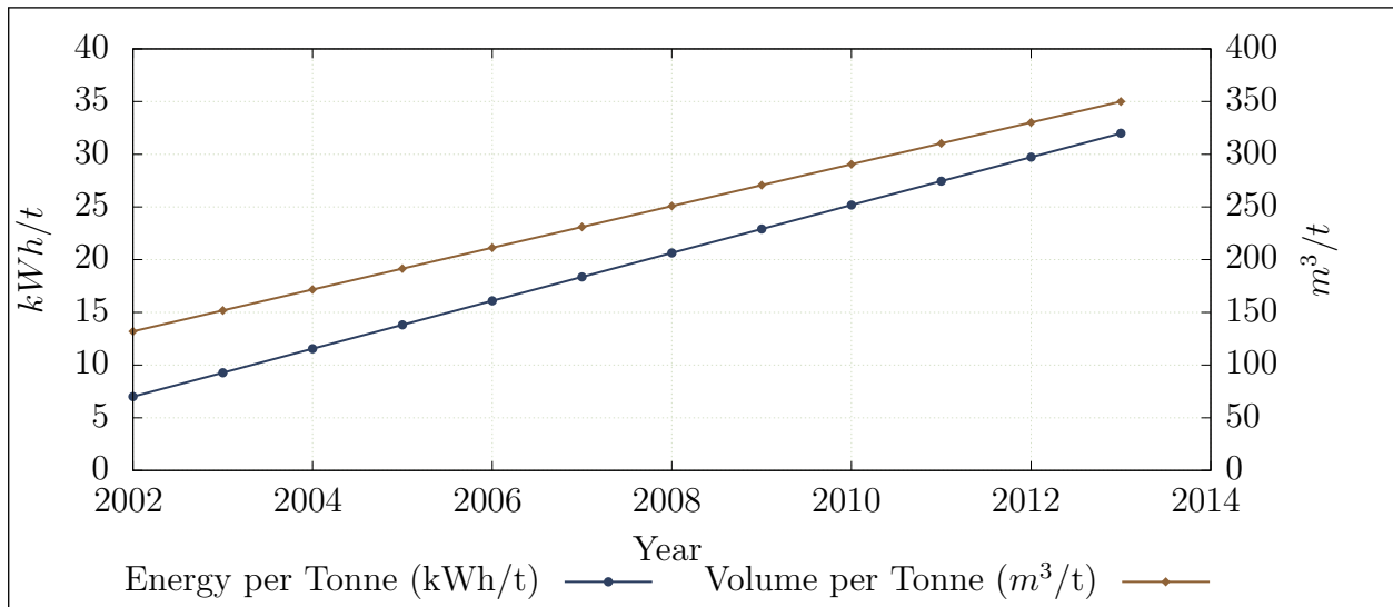
Figure 2.6: The compressed air energy and flow consumed per tonne of ore produced (adapted from Bester et al. [35])
