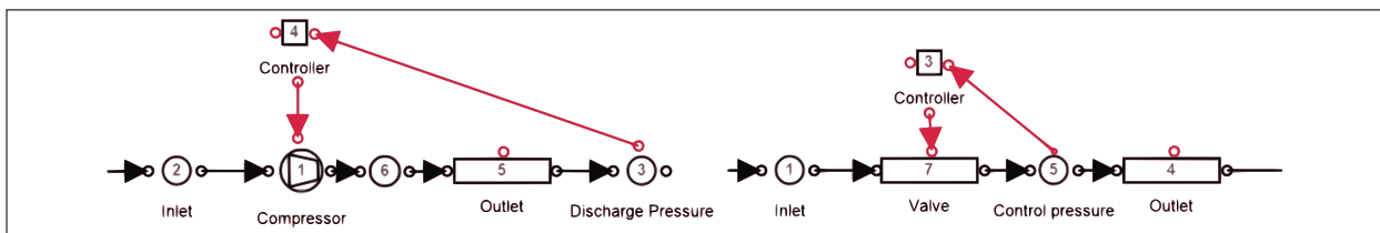
Figure 3.12: Control components in Process Toolbox
