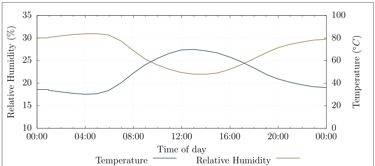
Figure 3.4: Average summer surface ambient air conditions at a South African gold mine
