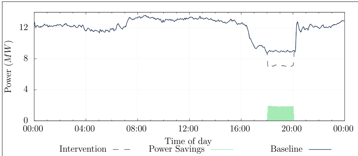
Figure 4.19: Energy saving achieved by general peak time station control
