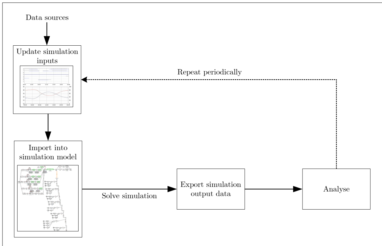
Figure 3.16: The periodic simulation process followed in this analysis
