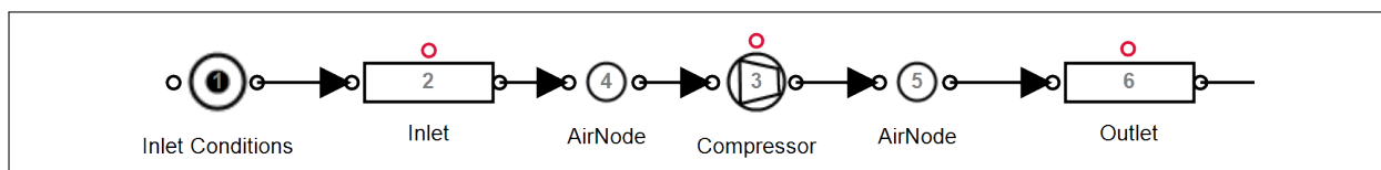
Figure 3.9: Integrating the compressor component into the simulation
