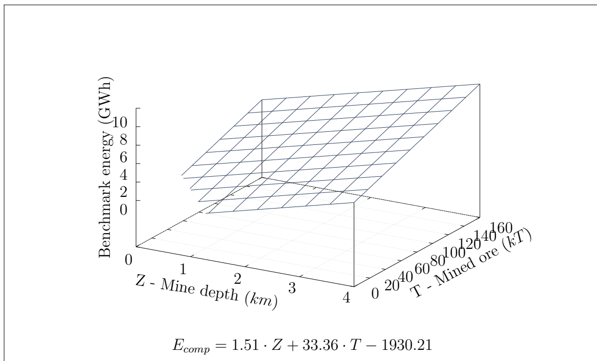
Figure 2.7: Energy benchmark model for a mining compressed air system (adapted from Cilliers [36])
