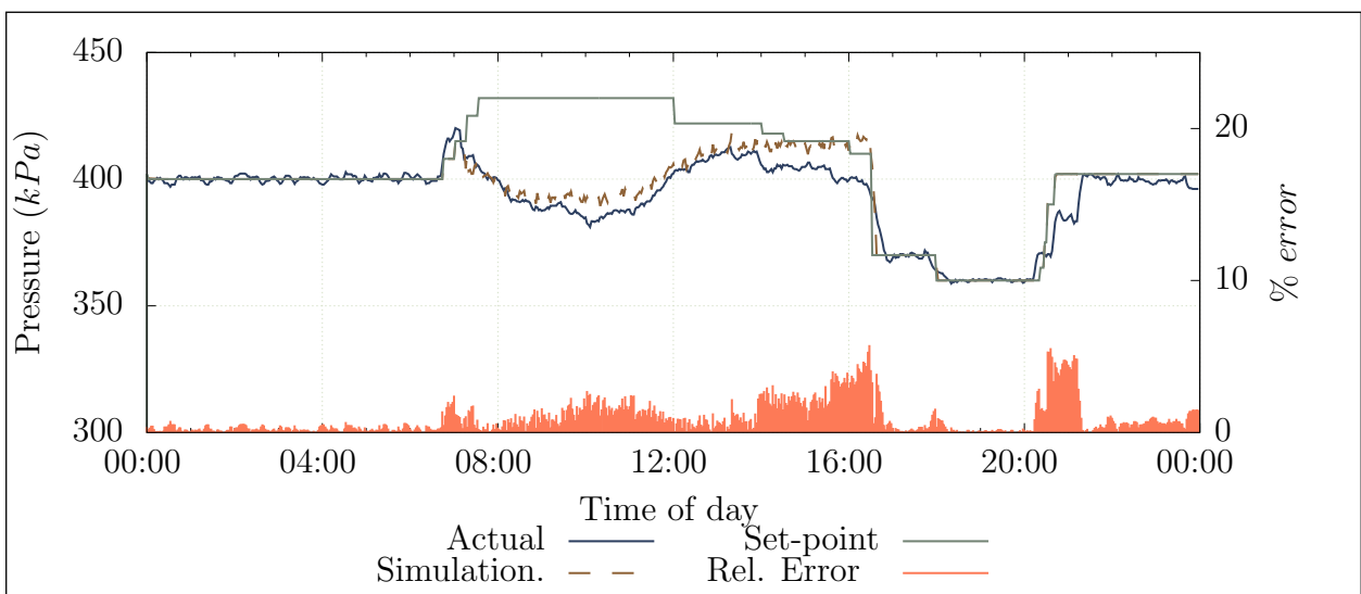
Figure 4.12: Simulated pressure compared to the actual measurement and set-points
