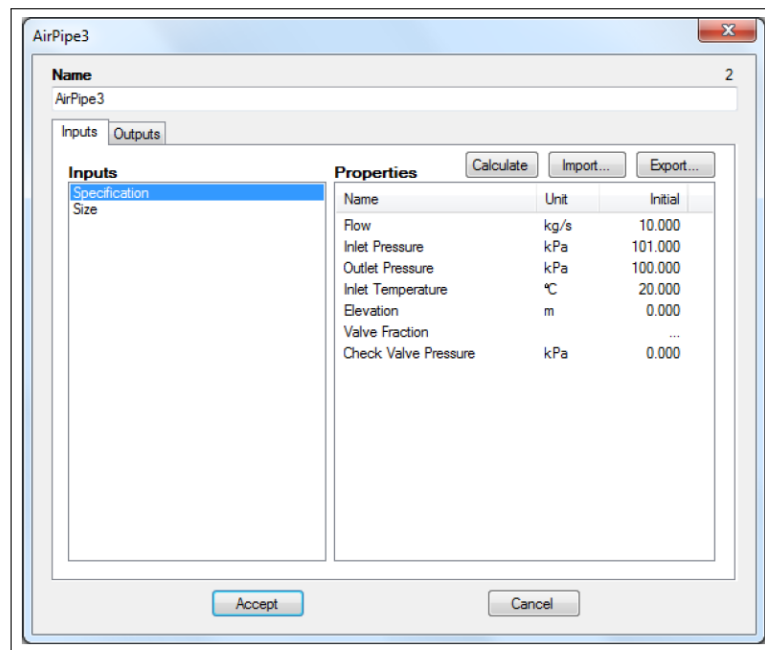
Figure 3.6: PTB air pipe configuration interface
