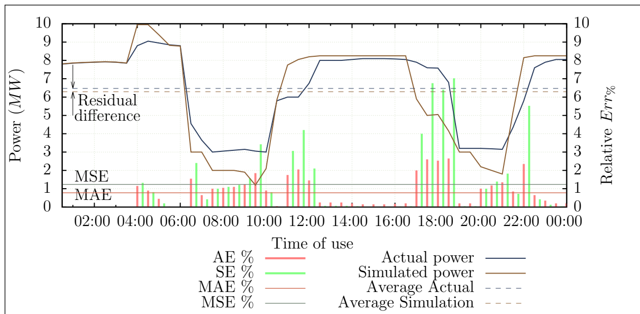
Figure 2.9: Example of simulation error calculations (data adapted from Maré [40])
