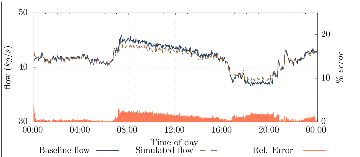
Figure 4.11: Simulated flow compared to the actual measurement
