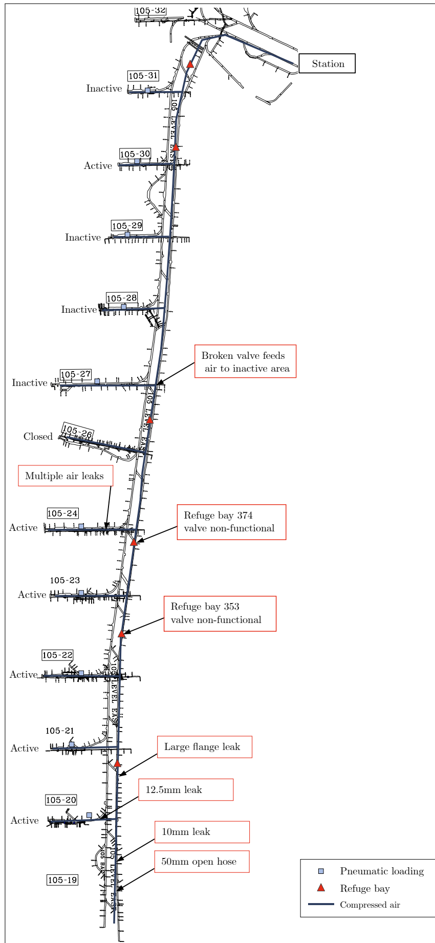
Figure IV.3: 105 Level investigation – East operation
