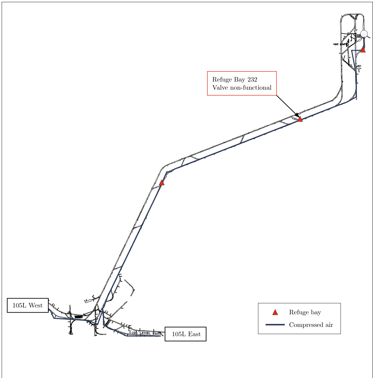
Figure IV.1: 105 Level investigation – Station
