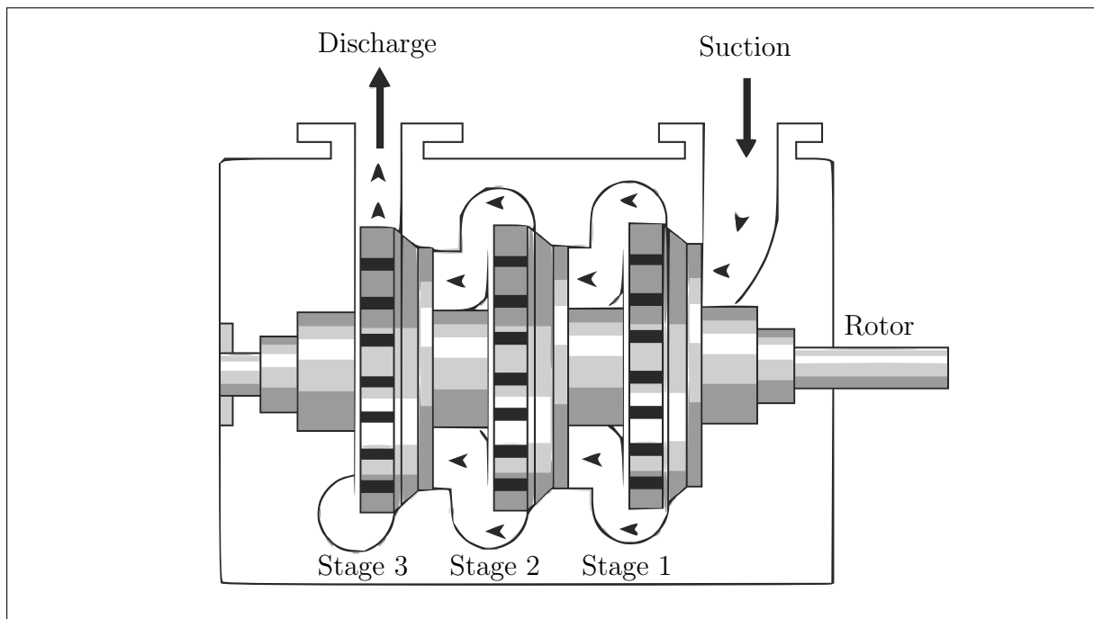
Figure 2.1: Schematic representation of a multi-stage centrifugal compressor 1
