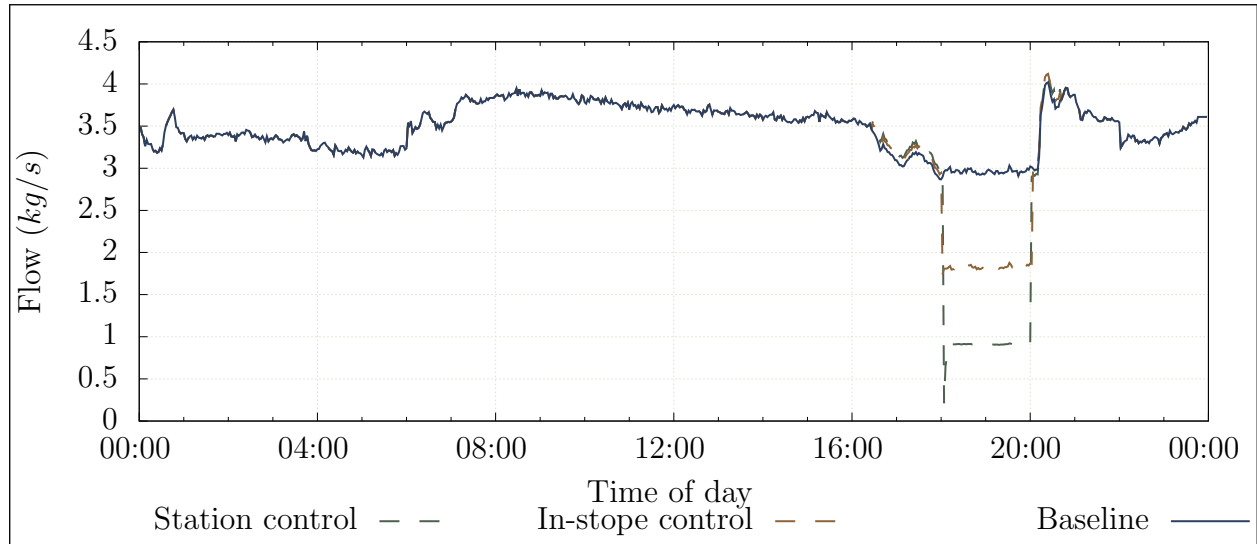
Figure 4.17: Flow reduction during blasting period for 105 Level
