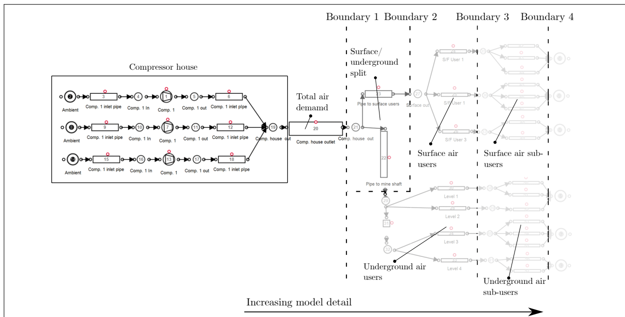
Figure 3.2: Selecting boundaries for the simulation model
