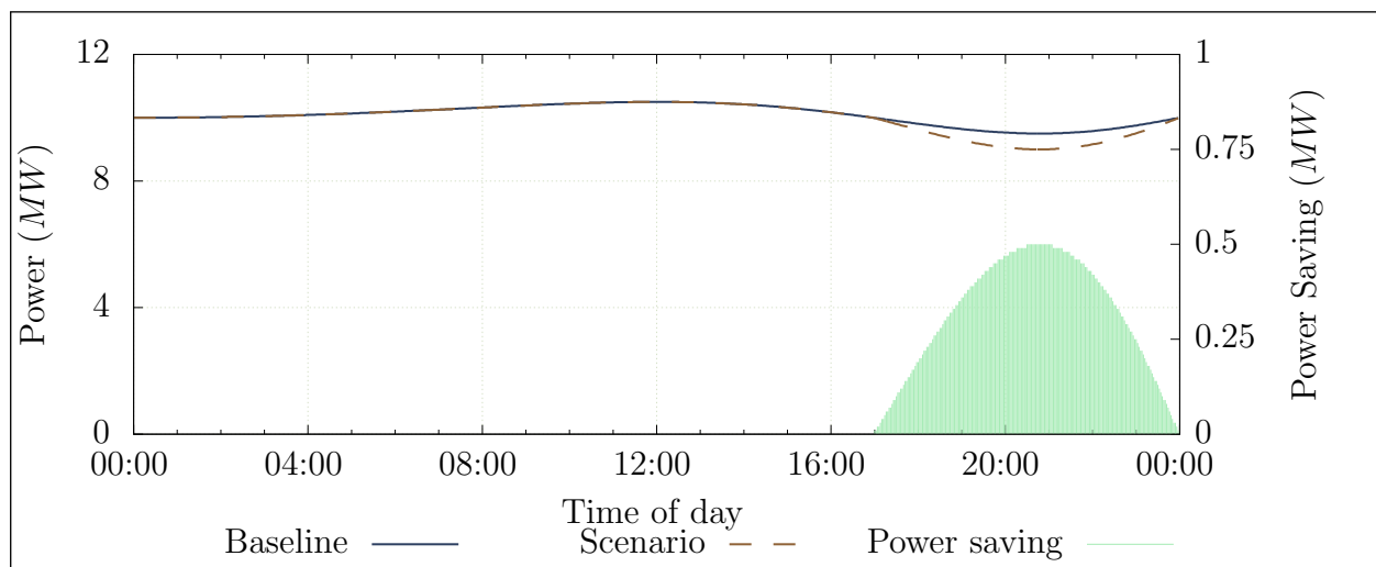
Figure 3.17: Theoretical example of a baseline vs. optimised power comparison
