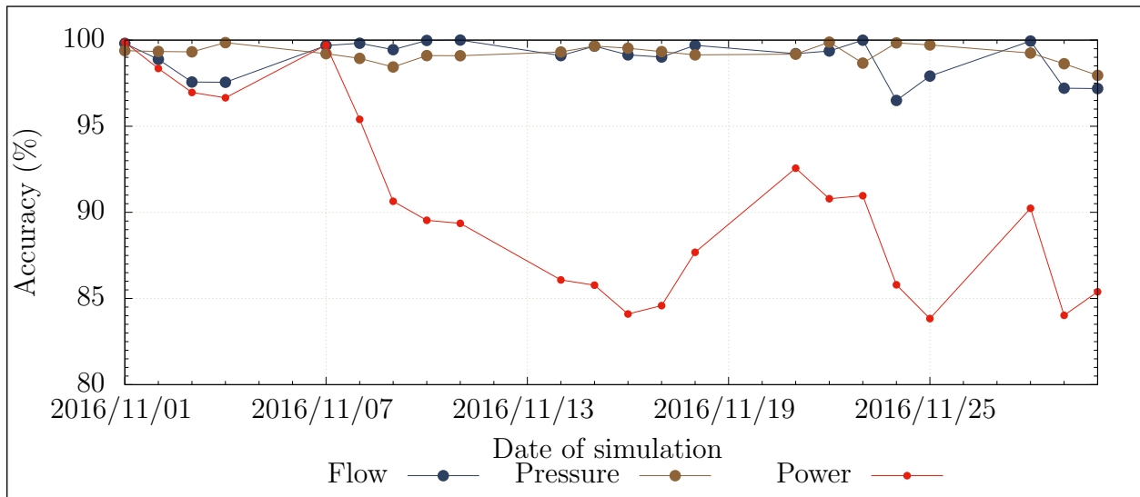
Figure 4.20: Flow, pressure and power error percentages for daily periodic simulations over a month
