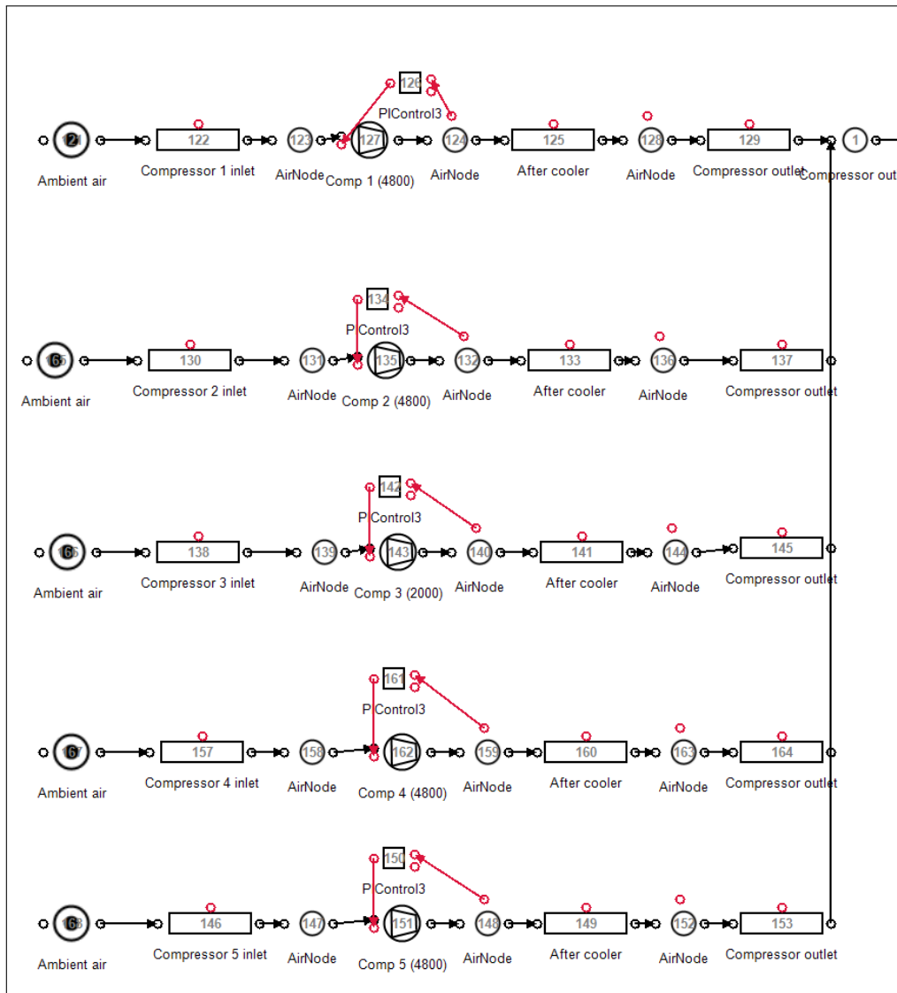
Figure I.3: Mine B simulation schematic – Compressors
