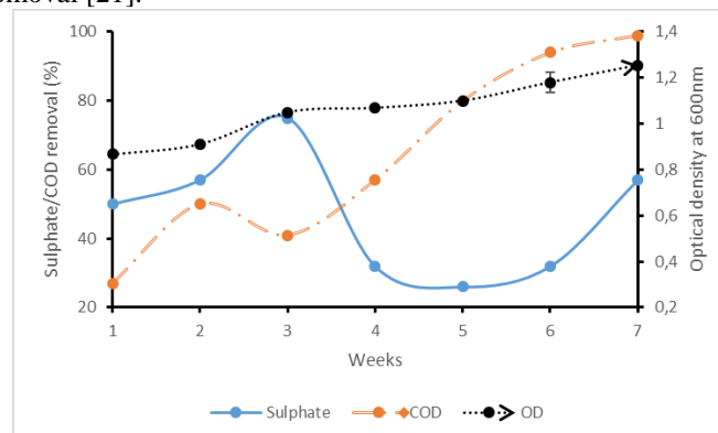
Fig. 1. Microbial growth with COD and Sulphate reduction in the anaerobic MBBR system.
