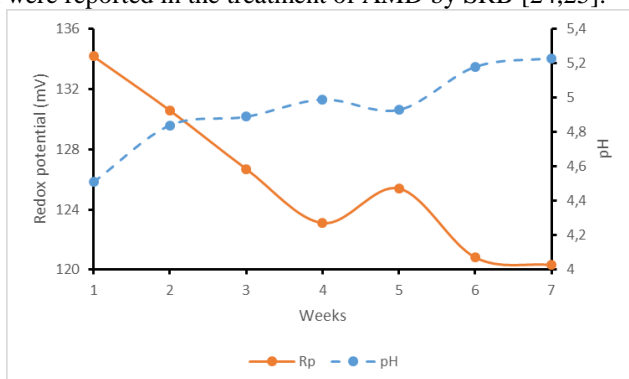
Fig. 2. Redox potential and pH of the SRB consortium in the anaerobic MBBR system.
