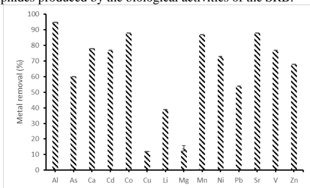
Fig. 3: Metal removal in the anaerobic MBBR system.
