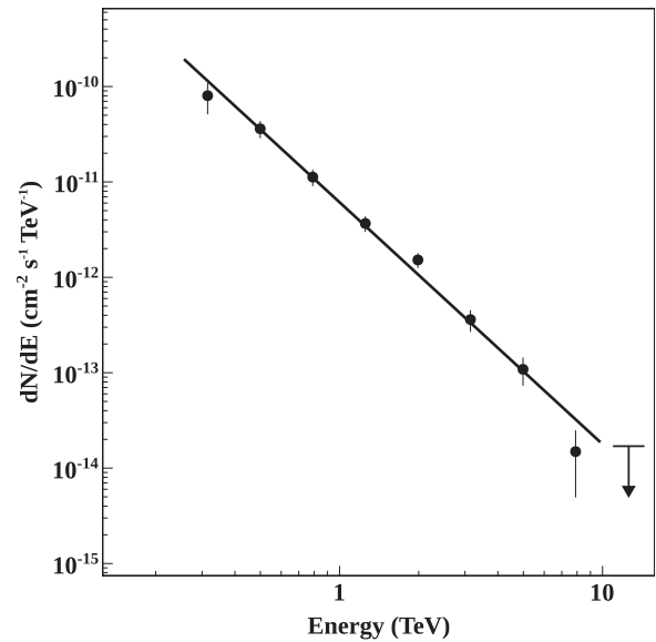
Figure 2. VERITAS time-averaged differential spectrum of 1ES 1959+650 fit with a power law of form dN/dE = N(E/E_0)^{-\Gamma} ; N = (6.12 \pm 0.53_{\text{stat}} \pm 2.45_{\text{sys}}) \times 10^{-12} \text{ cm}^{-2} \text{ s}^{-1} \text{ TeV}^{-1} , \Gamma = 2.54 \pm 0.08_{\text{stat}} \pm 0.3_{\text{sys}} , and E_0 = 1 \text{ TeV} .
